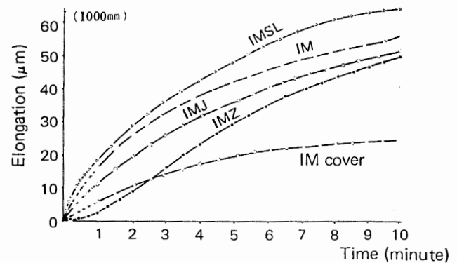
Fig. 11 Elongation by body heat
