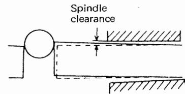
Fig. 2 Effect of excessive clearance
