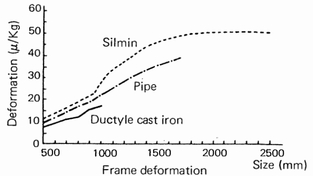
Fig. 6 Frame deformations of several materials
