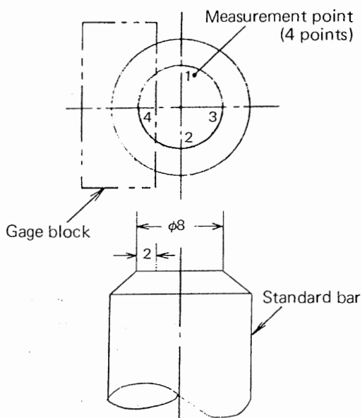
Fig. 1 Parallelism inspection
