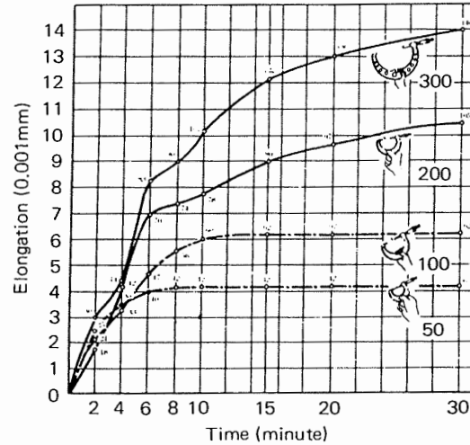
Fig. 5 Measurement error due to temperature variation
