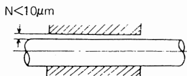
Fig. 1 Spindle clearance
