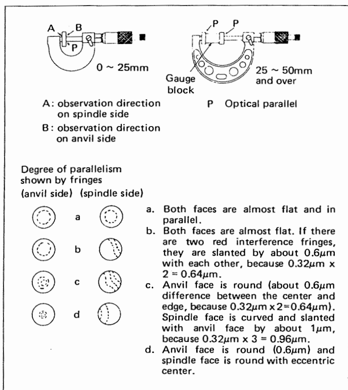
Fig. 4 Parallelism measurement
