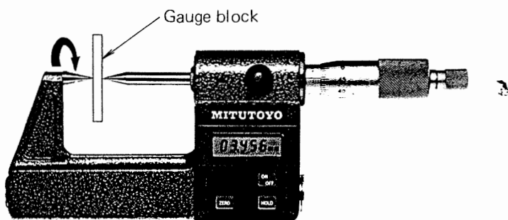
Fig. 3 Eccentricity inspection
