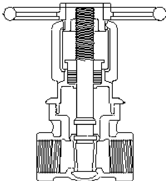
Figure 13.3 Rising stem gate valve.
