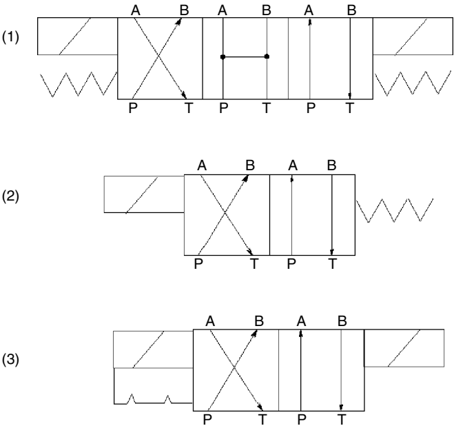
Figure 13.16 Actuator-controlled valve schematics.
