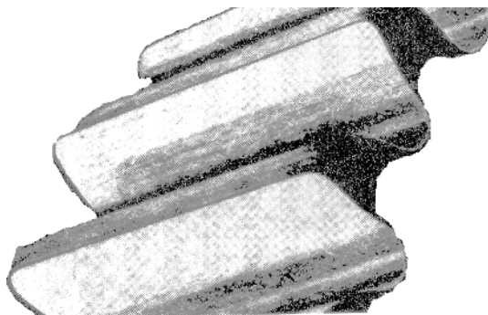
Figure 11.35 Normal wear pattern.
